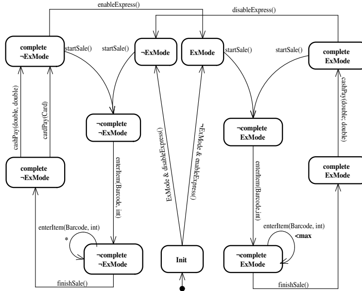
Figure 4: State diagram for UC 1 and 2
