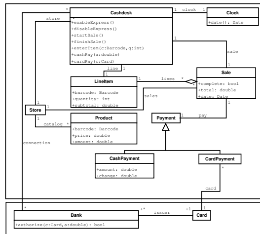
Figure 3: Use case class diagram for UC 1 &amp; 2
