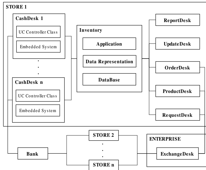
Figure 5: Overall component view of the system
