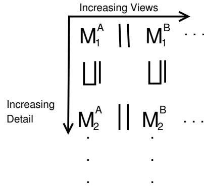
Figure 1: rCOS approach with views and refinements
