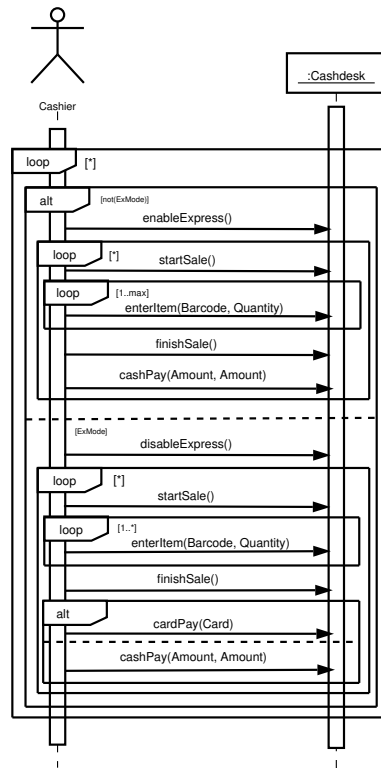
Figure 2: Use case sequence diagram for UC 1 & 2
