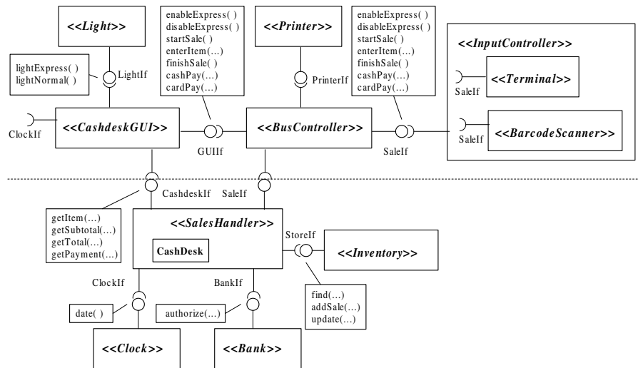
Figure 6: Deployed components for a single Cashdesk
