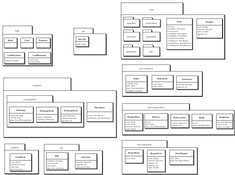
Fig. 8: Packages
